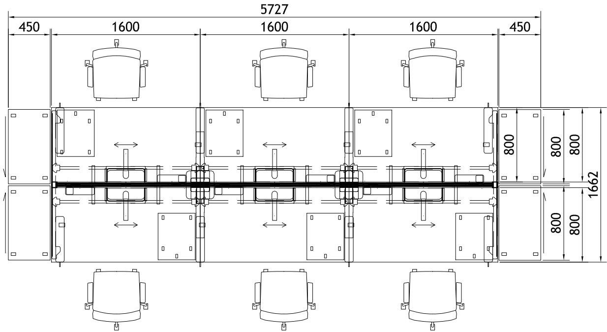
Plan View scale 1 : 40 mm
