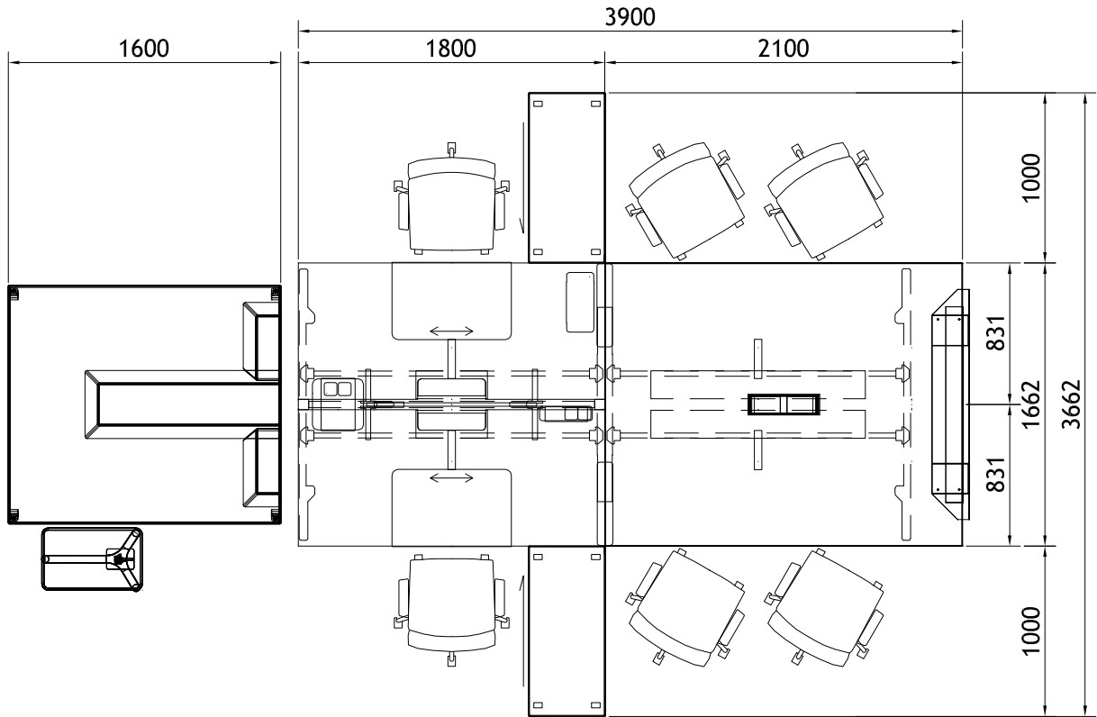
Plan View scale 1 : 40 mm
