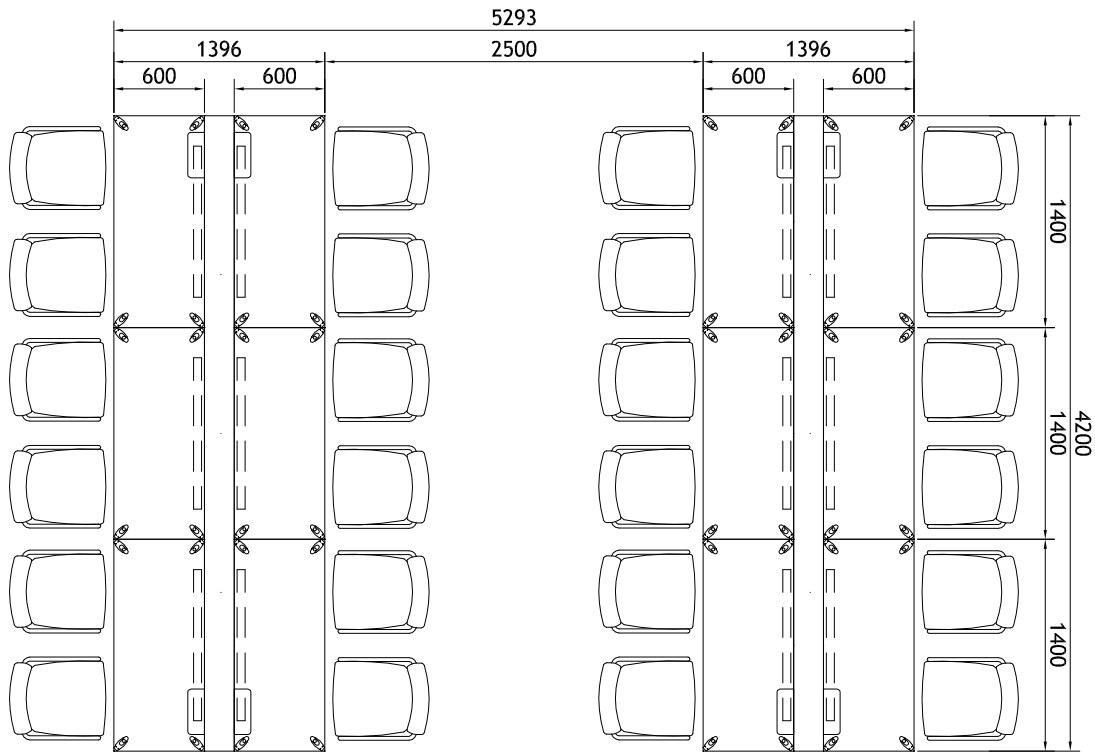
Plan View scale 1 : 50 mm
