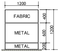
(A) INTERIOR SIDE
