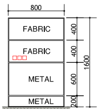
(B) BACK SIDE
