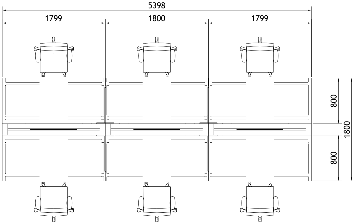
Plan View scale 1 : 40 mm
