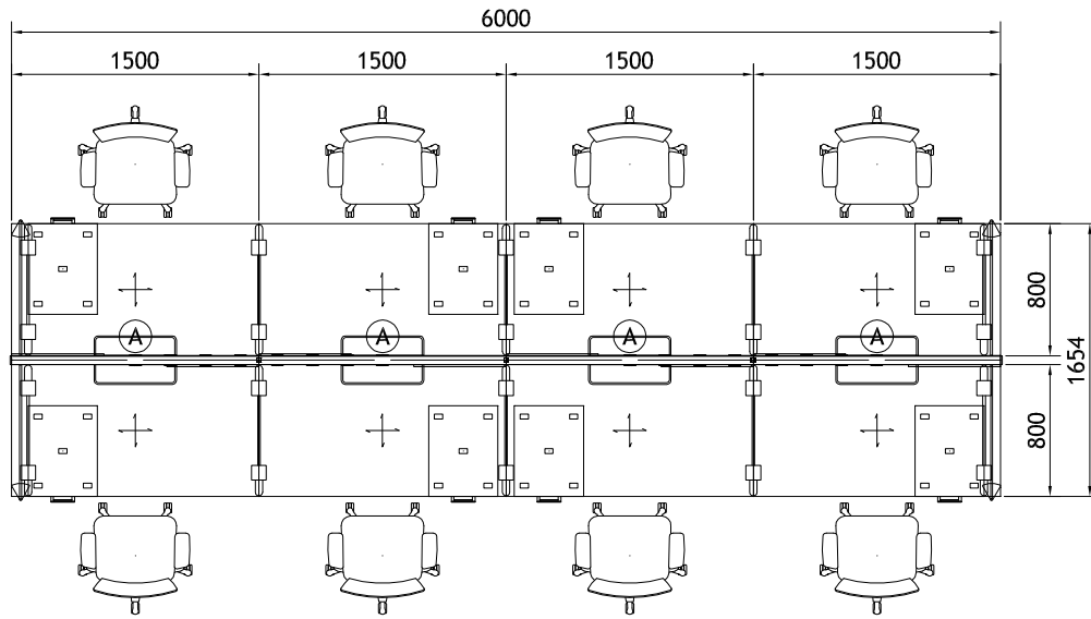
Plan View scale 1 : 50 mm
