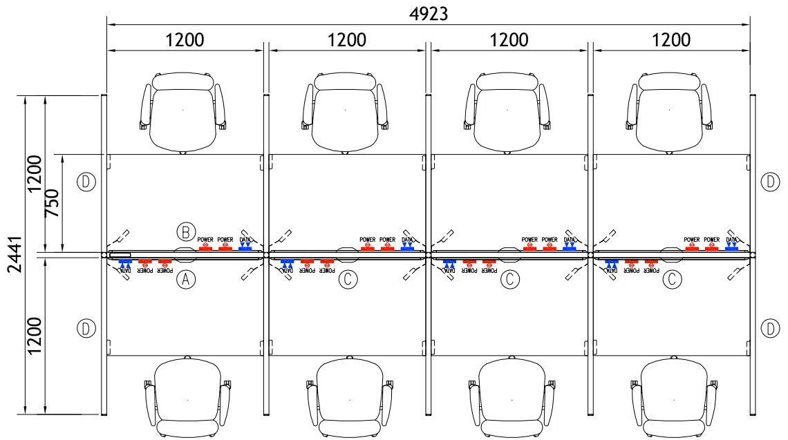
Plan View scale 1 : 40 mm
