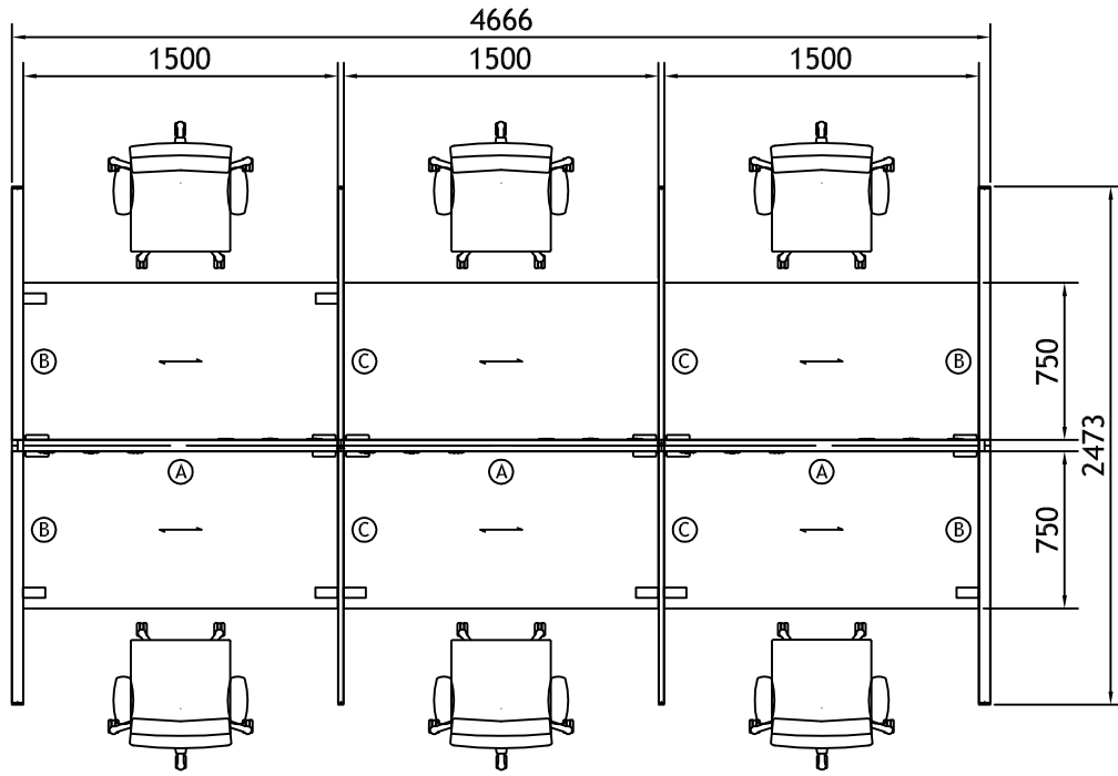
Plan View scale 1 : 40 mm
